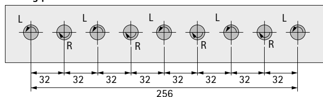
Drilling pattern
