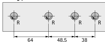
Drilling pattern
