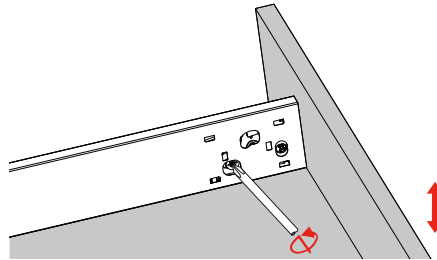
Height adjustment
