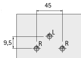
Drilling pattern
