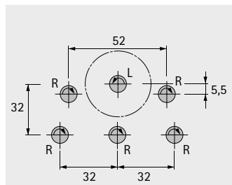
Drilling pattern
